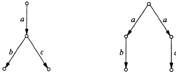
FIG. 13. Completed trace equivalent but not de Simone congruent.
