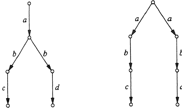
FIG. 14. de Simone congruent but not GSOS congruent.
